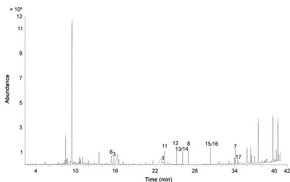
Fig. 8. TIC of Achillea millefolium obtained using GC–EI–MS.
