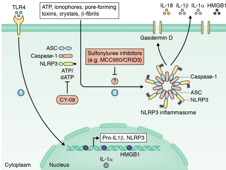
Activation of the NLRP3 inflammasome and its inhibition by CY-09 and sulfonylurea compounds. Activation of the NLRP3 inflammasome involves two steps. First, TLR4 stimulation induces transcriptional up-regulation of NLRP3 and the inflammasome substrate proIL-1 \beta . In the second activation step, NLRP3 agonists such as ATP, the ionophore nigericin, pore-forming toxins and internalized crystals, and \beta -fibrils trigger NLRP3 oligomerization, ASC speck formation, and inflammasome-mediated caspase-1 autoactivation. Caspase-1 cleaves its cytokine substrates IL-1 \beta and IL-18, and it induces pyroptosis through cleavage of gasdermin D, which promotes the passive release of IL-1 \beta and IL-18 along with DAMPs such as IL-1 \alpha and HMGB1. CY-09 inhibits NLRP3 inflammasome assembly by blocking ATP/dATP binding in the central NACHT domain, whereas the target and mechanism of action of sulfonylurea compound MCC950/CRID3 are unknown.
