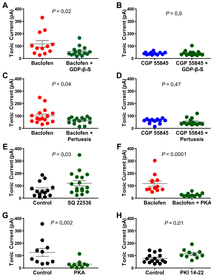
Figure 3. Recordings from TC neurons shows that baclofen enhances tonic GABA A -mediated currents through a G 1/0 G-protein, adenylate cyclase, and PKA-dependent pathway. A , Blockade of all G-protein signaling with GDP-β-S (1 mM) prevented the baclofen-induced enhancement in tonic current. B , GDP-β-S (1 mM) does not block the tonic current directly, as in the presence of CGP 55845 (1 μM) GDP-β-S has no effect on the magnitude of the tonic current. C , Blocking all G i dependent G-protein signaling with pertussis toxin (500 ng/ml) prevented the baclofen-induced enhancement in tonic current. D , Pertussis toxin does not block the tonic current directly, as it did not reduce the amplitude of the tonic current when applied together with CGP 55845 (1 μM). E , The inhibitor of adenylate cyclase SQ 22536 (10 μM), mimicked the effect of baclofen and enhanced the tonic current. F , Infusion of the active catalytic subunit of PKA (10 IU/ml) blocked the enhancement of the tonic current caused by baclofen. G , PKA (10 IU/ml) significantly reduced the tonic current. H , The PKA inhibitor PKI 14-22 (50 ng/ml) mimicked the effect of baclofen and produced significant enhancement of GABA A receptor-mediated tonic current.
