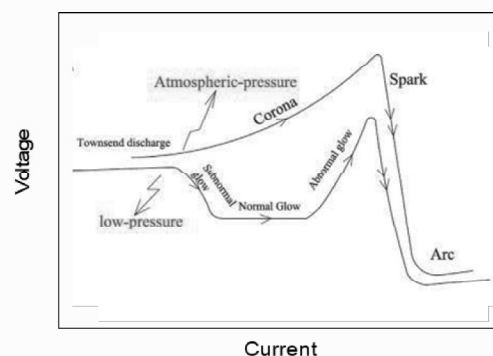
Figure 1. Schematic current-voltage characteristics of the different types of discharges in gases.
