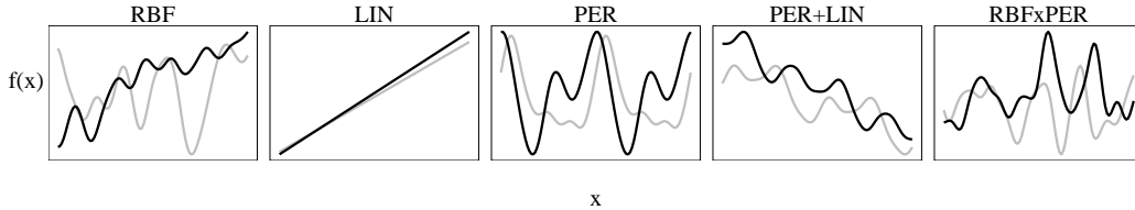
Figure 1. Examples of base and compositional kernels. The base kernels are radial basis ( RBF ), linear ( LIN ), and periodic ( PER ); the composition operators are addition and multiplication. Adding a periodic and a linear kernel creates functions with trends and seasonality. Multiplying a periodic kernel with a radial basis kernel results in more localized periods than a standard periodic kernel would be able to capture.
