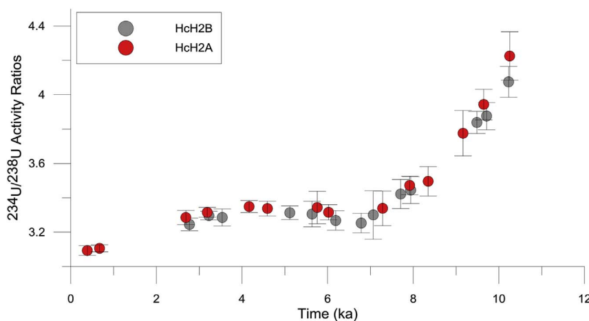
Fig. 6. Initial ^{234}\text{U}/^{238}\text{U} activity ratios for coeval stalagmites HcH2B (grey) and HcH2A (red) are plotted against age. Error bars signify a 2\sigma uncertainty. (For interpretation of the references to colour in this figure legend, the reader is referred to the web version of this article.)
