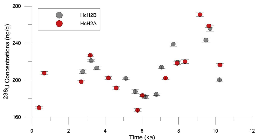
Fig. 5. ^{238}\text{U} concentrations for coeval stalagmites HcH2B (grey) and HcH2A (red) are plotted against age. Error bars signify 2\sigma uncertainty. (For interpretation of the references to colour in this figure legend, the reader is referred to the web version of this article.)
