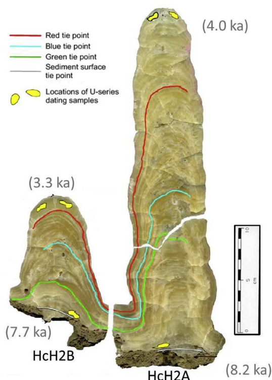
Fig. 1. Stratigraphic correlation tie point locations, shown in green, blue and red. Sample positions for preliminary U-Th dates are in yellow. Bracketed values are provisional dates calculated in 2005, which suggested a likely Holocene age and possibly coeval growth for both stalagmites. They are not used further in this paper. (For interpretation of the references to colour in this figure legend, the reader is referred to the web version of this article.)
