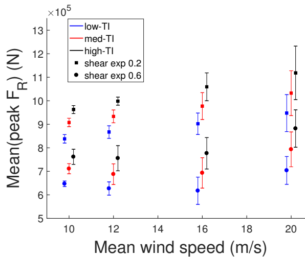
Figure 6. Mean peak radial loading over each set of six wind fields with parameters in common. Note, results have been staggered about each mean wind speed for clarity.
