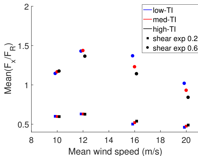
Figure 5. Mean axial to radial load ratios. Note, results have been staggered about each mean wind speed for clarity.
