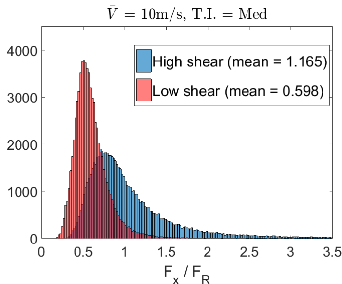
Figure 4. Histogram of axial to radial bearing reaction force ratios across simulations with a mean wind speed of 10m/s, medium turbulence intensity and low (0.2) and high (0.6) shear exponents.
