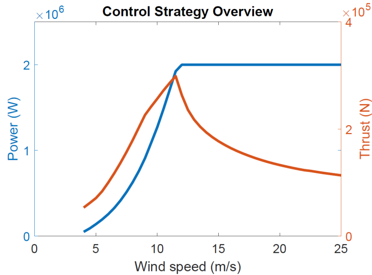
Figure 1. Design power and thrust curves for the simulated wind turbine.
