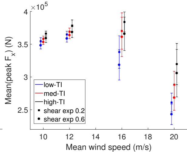
Figure 7. Mean peak axial loading over each set of six wind fields with parameters in common. Note, results have been staggered about each mean wind speed for clarity.
