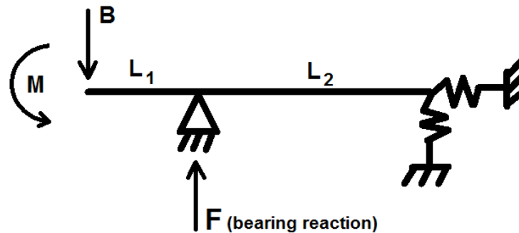
Figure 3. Simplified drivetrain model for each in-plane force-moment pair.
