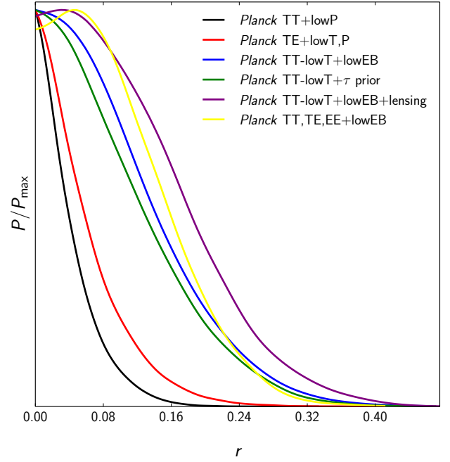
Fig. 8. One-dimensional posterior probabilities for r for various data combinations, either including or not including temperature multipoles for \ell < 30 , and compared with the baseline choice ( Planck TT+lowP, black curve).
