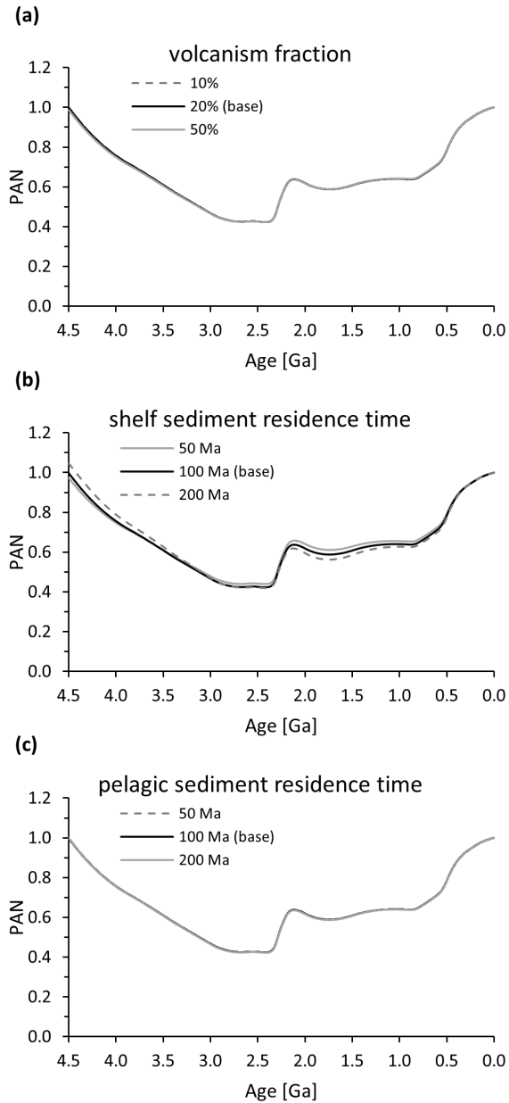
Figure A6: Sensitivity tests, second batch. Parameters were changed individually while keeping all other parameters equal to base values. Calculations are based on the “ F_{org} + Heatflow” model.
