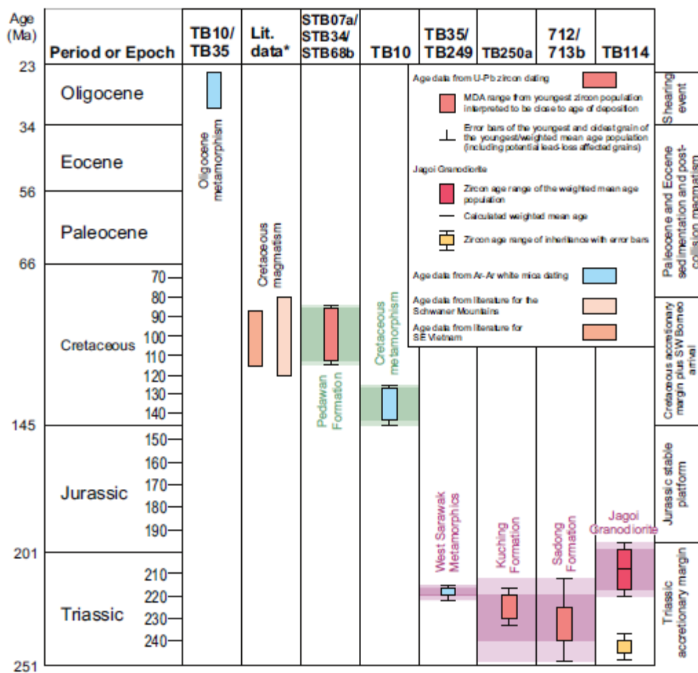
Fig. 13: Summary of magmatic and metamorphic ages from the accretionary margin in West Sarawak and NW Kalimantan. Data from the Schwaner Mountains of the SW Borneo block from Haile et al. (1977), Williams et al. (1988), van Hattum et al. (2013) and Davies et al. (2014). Data from SE Vietnam from Nguyen et al. (2004) and Shellnutt et al. (2013).
