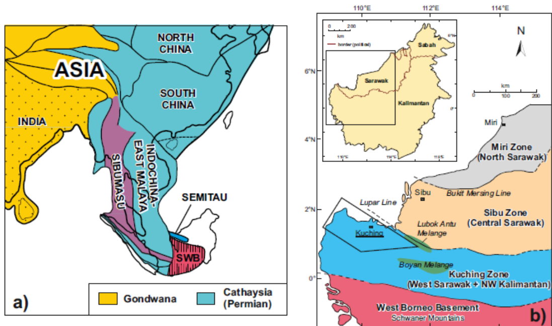
Fig. 1: a) Principal continental blocks of SE Asia showing the interpreted Semitau and SW Borneo (SWB) blocks (modified after Metcalfe, 2013). Sibumasu and Indochina-East Malaya formed Early Mesozoic Sundaland. b) Tectonic provinces of NW Borneo (modified after Haile, 1974). The black box shows the research area in the Kuching Zone (West Sarawak).
