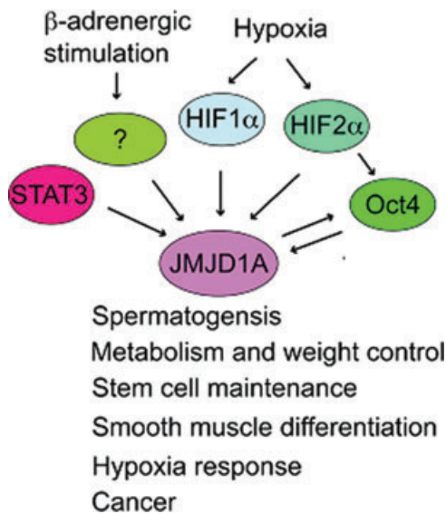
Figure 6. Potential roles of JMJD1A.
