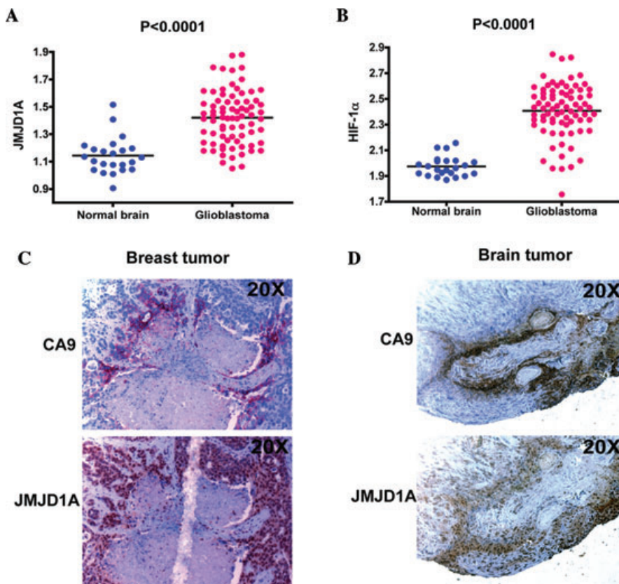
Figure 4. JMJD1A expression is associated with hypoxia in cancer. ( A, B ) JMJD1A and HIF-1 \alpha data from the Sun et al. study 53 were reanalyzed using the Prism program. ( C, D ) JMJD1A expression in breast cancer and glioblastoma samples were analyzed using immunohistochemistry (magnification \times 20 ).
