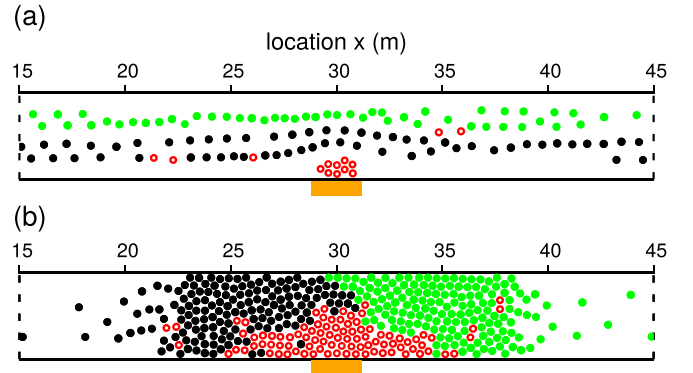
FIG. 1. Representative snapshots of different passerby flow patterns, showing a section of 30 m in the center of the corridor, i.e., 15 \text{ m} \leq x \leq 45 \text{ m} . The attraction, depicted by an orange rectangle, is located at the center of the lower wall with open boundary conditions in the horizontal direction. Closed black and green circles indicate passersby walking to the right and to the left, respectively. Open red circles depict pedestrians attracted by the attraction. In bidirectional flow, we can observe (a) the free flow phase in the case of Q = 4 \text{ P/s} and s = 0.5 , in which passersby can walk towards their destinations without being interrupted by the cluster of attracted pedestrians, and (b) the freezing phase in the case of Q = 4 \text{ P/s} and s = 1 , where oppositely walking pedestrians stopped because they block each other. Note that P/s stands for pedestrians per second, being the unit of pedestrian flux Q .
