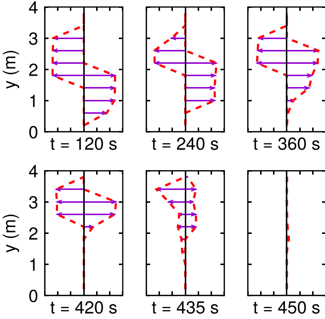
FIG. 10. Streamwise velocity profiles of passerb traffic in the corridor at x = 30 m with Q = 4 P/s and s = 1 in bidirectional flow. Based on Eq. (F3), the velocity vectors are presented for eastbound and westbound passerb traffic in the right and left parts of each panel, respectively. In the course time, the velocity profile curves are gradually shifting upward while their magnitude decreases.
