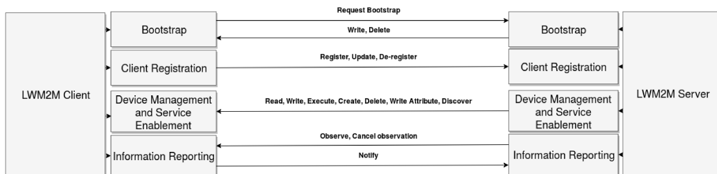
Figure 2.2: LWM2M Interfaces
