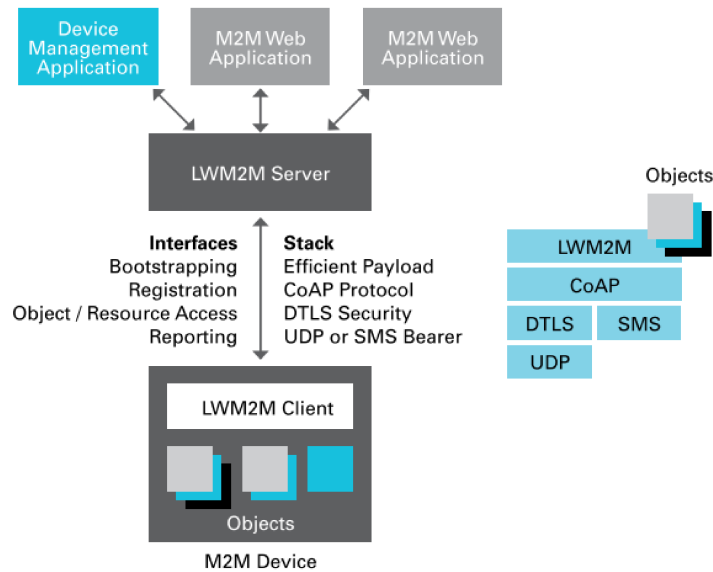
Figure 2.1: LWM2M Architecture
