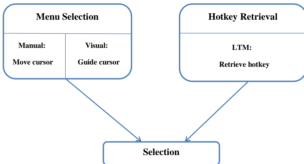
Figure 7: The threads and resources of menu selection and hotkey retrieval
