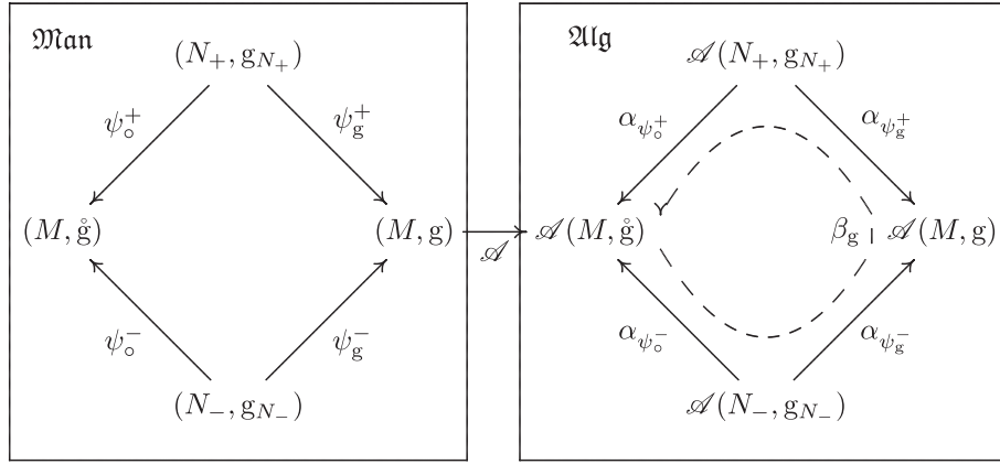
FIG. 2. Diagram of the perturbed spacetime, along with the embedded subregions N_{\pm} , the locally covariant quantum field theory thereon, and the relevant morphisms, where \mathring{g} = g^{(0)} and g = g^{(s)} .
