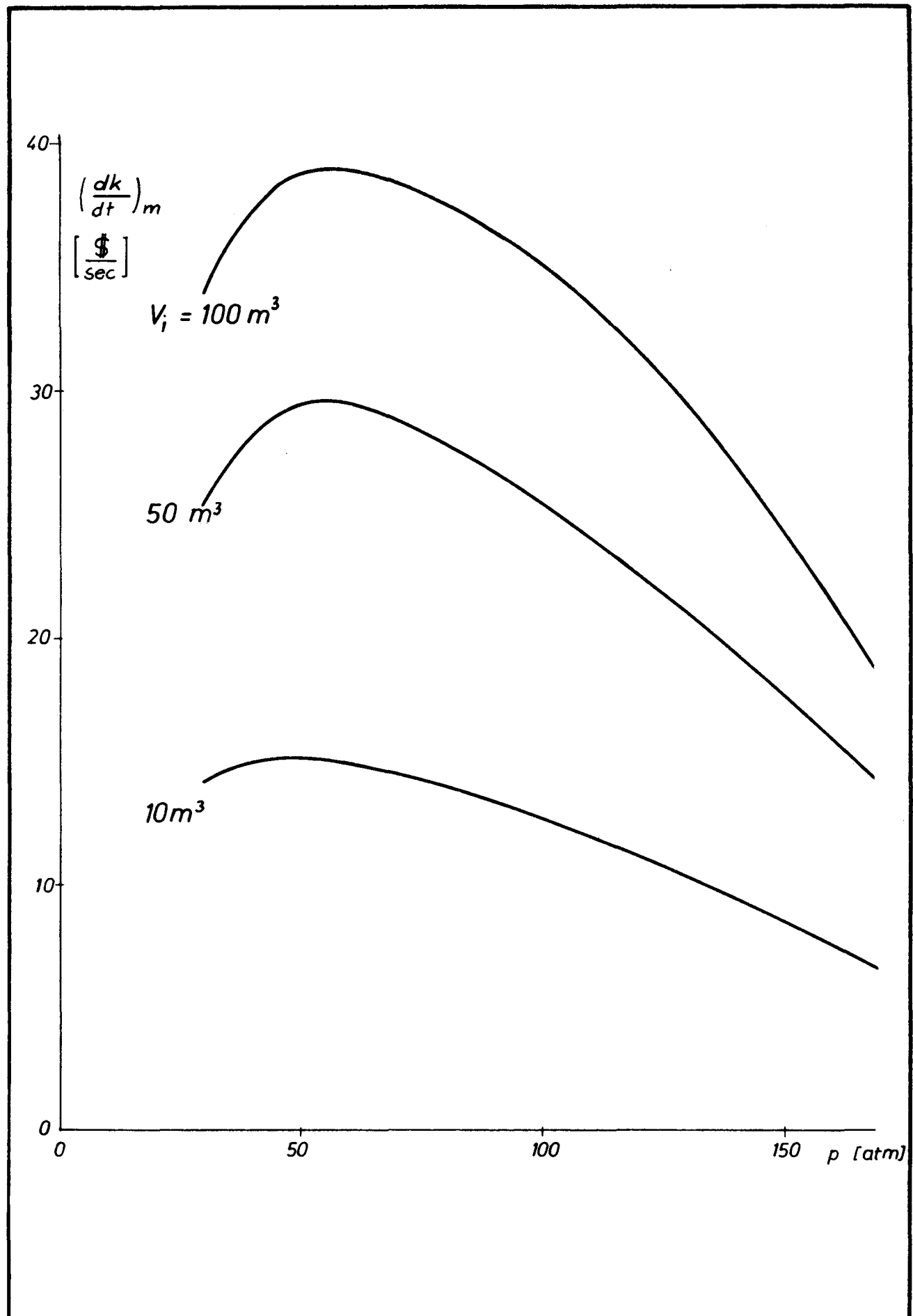
Fig. 20 Reactivity rate of unflooding accident as influenced by the pressure
