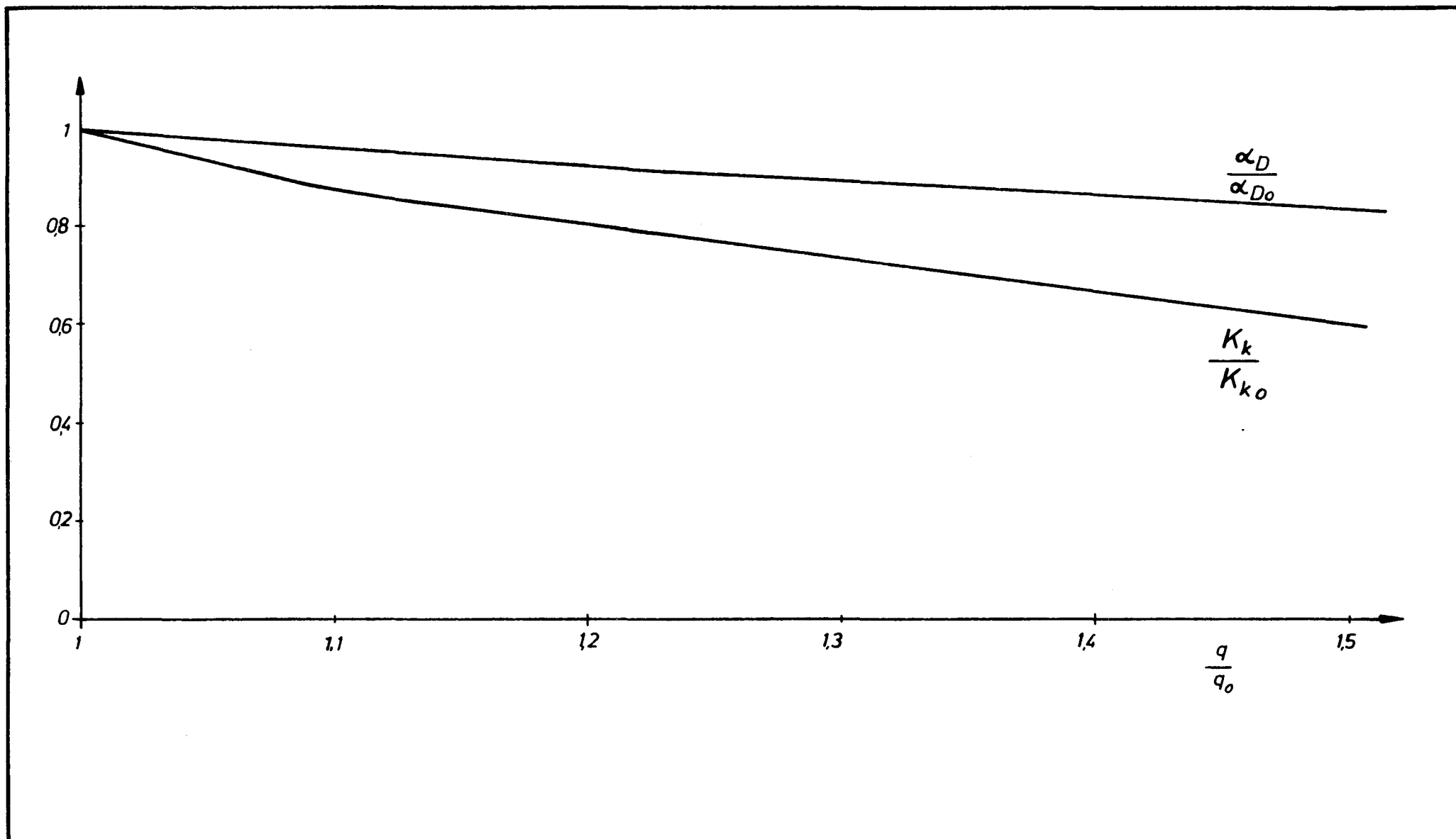
Fig.3 Relative changes of Doppler coefficient and reactivity gain versus rod power
