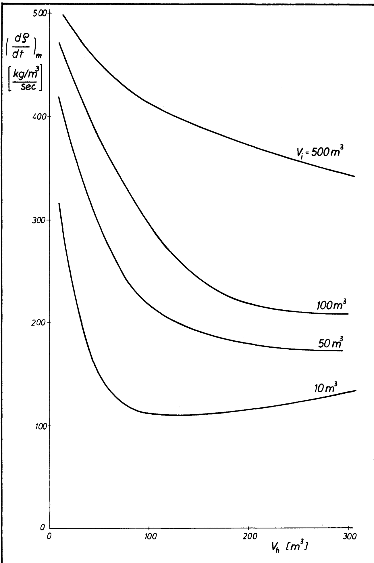
Fig.21 Density reduction rate of unflooding accident as influenced by the volumes
