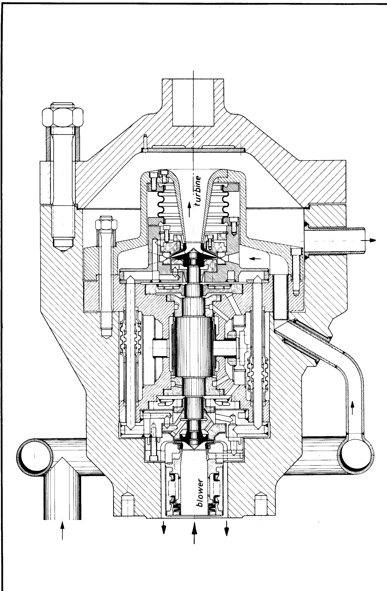
Fig.7 Turbine driven steam blower
