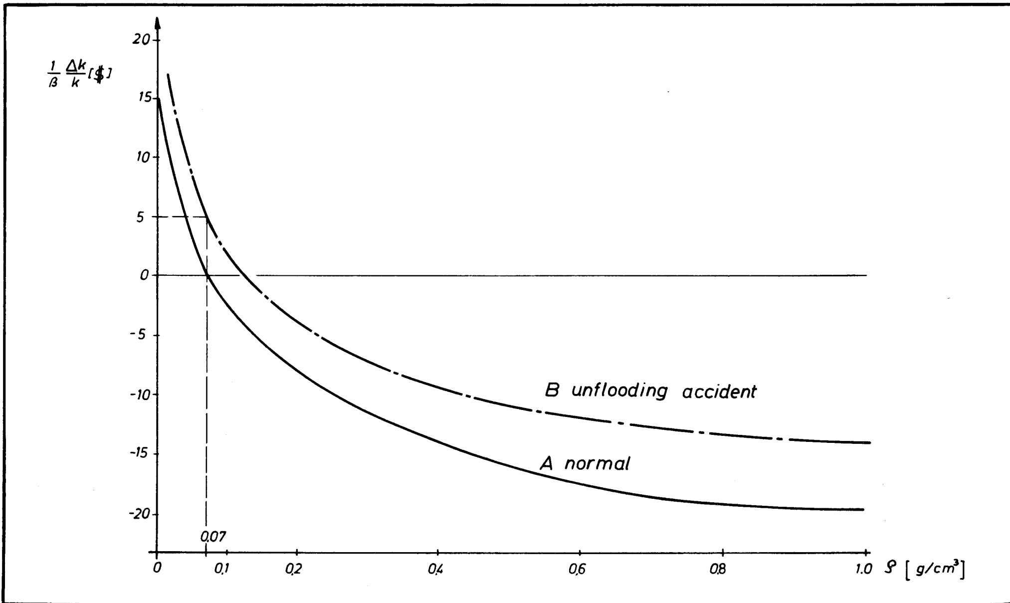
Reactivity versus steam density
