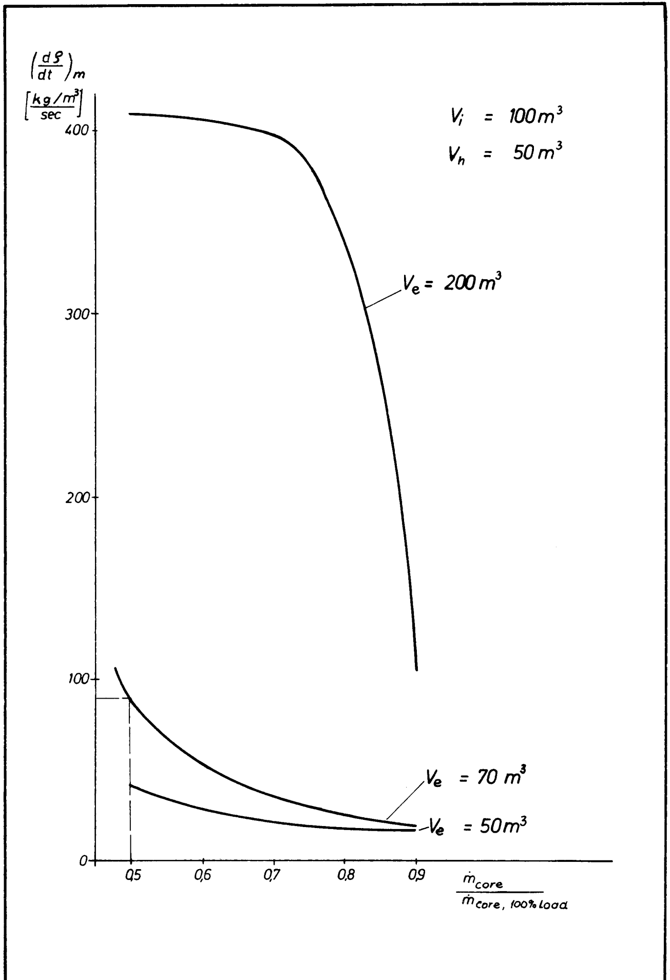
Fig. 12 Density reduction rate as caused by rupture of saturated steam pipe at 50% load
