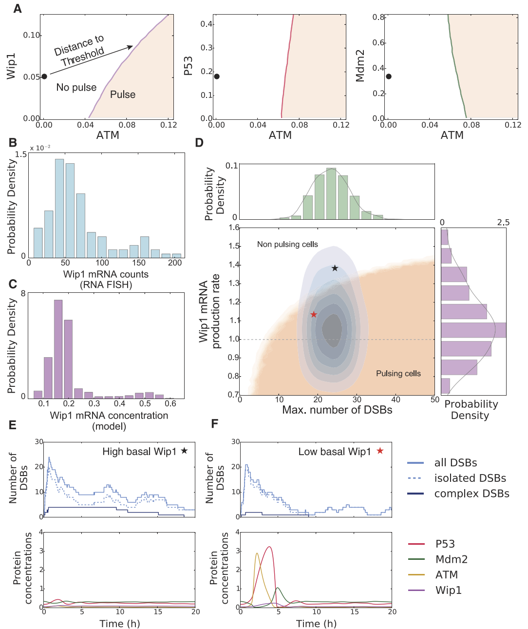
Figure 4. The responsiveness of individual cells towards damage is modulated by Wip1 levels. (A) Sensitivity of the excitation threshold for fluctuations of the three regulated proteins p53, Mdm2 and Wip1. The steady state is depicted as (●) for basal activated ATM levels on the left respectively. The p53 system is particularly sensitive to Wip1 fluctuations, as it influences the threshold the most. (B) Measured single cell Wip1 mRNA counts for an unstimulated cell population ( N = 106 ). (C) Modeled in silico Wip1 mRNA concentration variability. The single cell expression levels were drawn from a log-normal distribution and the system was driven by basal DSB dynamics. (D–F) The dependency of p53 responsiveness on damage levels (maximal number of inflicted DSBs) and Wip1 expression rate is shown in D. Cells responding with a p53 pulse lie inside the beige area. A typical fixed dose experiment will induce a distribution of cells inside this plane (blue contours), as both the number of DSBs and the Wip1 expression levels are variable on the single cell level. The fraction of cells within the beige area determines the population response. Exemplary simulations of cells with high (E, black star) or low (F, red star) Wip1 are shown. Although both cells suffered comparable numbers of DSBs, only the cell with low Wip1 level was responsive.
