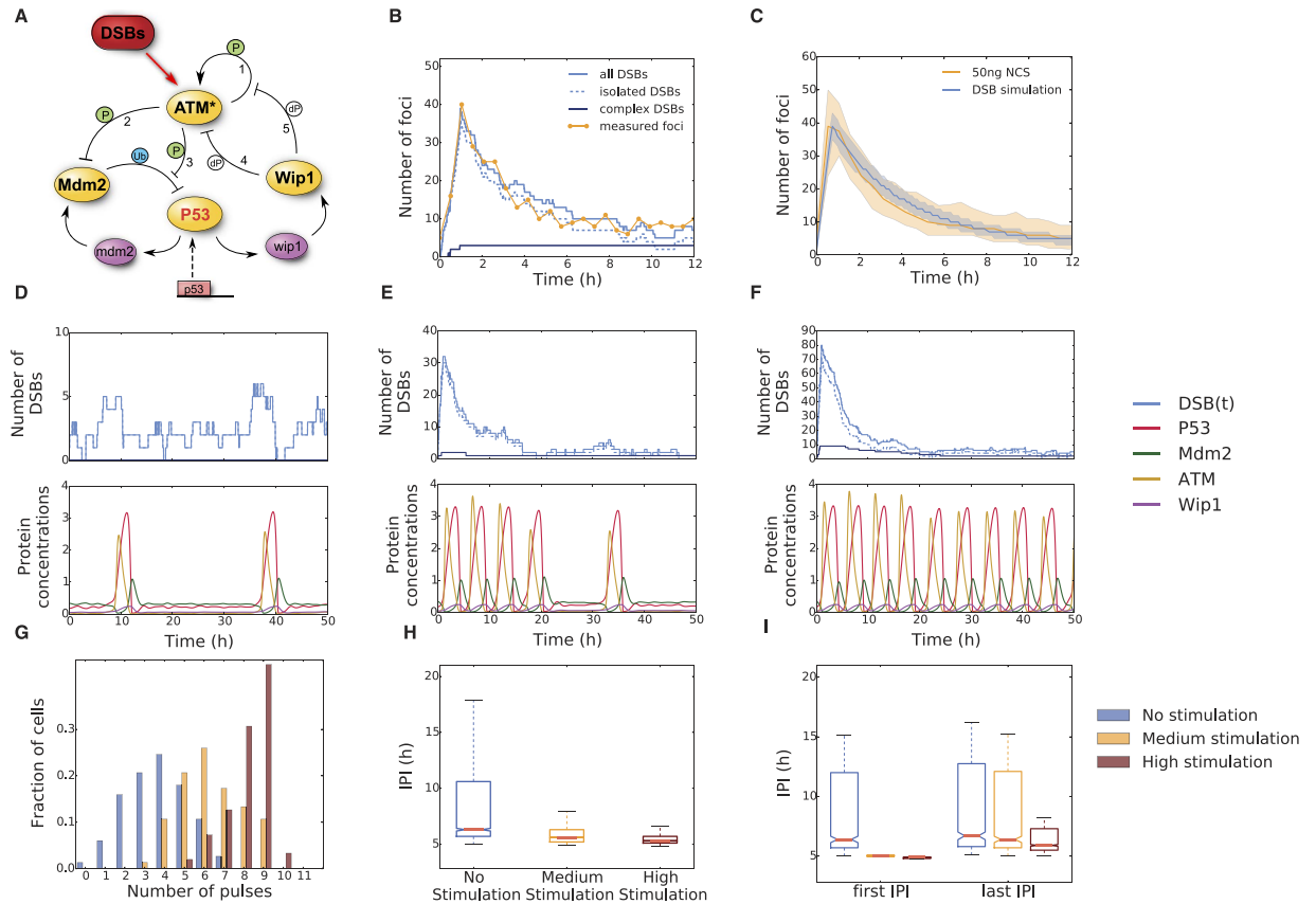
Figure 3. A p53 model driven by stochastic DSB processes recovers experimentally measured dynamical properties. (A) Interaction graph of the modeled p53 network in response to DSBs. Modelled molecular interactions include phosphorylation (P), dephosphorylation (dP) and ubiquitination (Ub); mRNA species (mdm2 and wip1) are shown in purple, all other species describe proteins. The numbers refer to the explanations in the text. (B) A single exemplary realization of the stochastic DSB process. Shown are the dynamics of the two damage types (isolated and complex) and the total effective number of DSBs over time. For comparison, the measured number of DSBs over time post damage is shown for an individual cell (yellow). (C) Statistics of measured and simulated foci for populations of cells. Shown are the median and 1 st and 3 rd quartiles. N = 120 for simulations, N = 52 for measurements. (D–F) Exemplary DSB process realizations and the corresponding p53 model responses. Shown are three different stimulus intensities: control condition (D), medium stimulation (E) and high stimulation (F). (G) Pulse counting statistics for three simulated ensembles with stimulation strengths as indicated. (H) Inter-pulse-interval (IPI) distributions corresponding to the ensembles shown in G. The overall coherence of the pulsatile response increases with stimulation strengths. (I) First and last IPI distributions for the three different stimulation strengths corresponding to the simulated ensembles shown in G and H. The medium stimulated cells have mostly returned to unstimulated dynamics, whereas the highly stimulated cells still predominantly show coherent oscillations on the single cell level.
