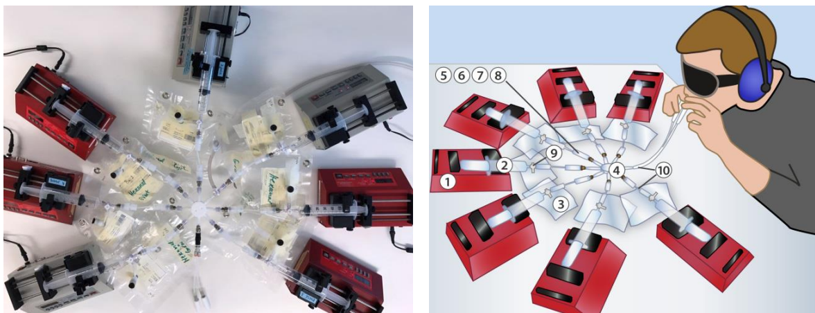
Figure 8: The olfactometer
