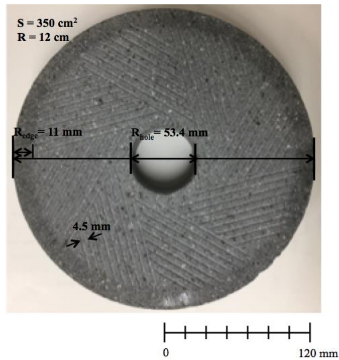
Fig. 2. The lower millstone of the Mill with contact surface area of 350 \text{ cm}^2 , millstone radius of 12 \text{ cm} , edge distance of 11 \text{ mm} , and groove width of 4.5 \text{ mm} . The upper millstone is the same as the lower millstone.
