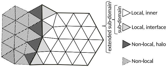
Fig. 3. Domain decomposition.
