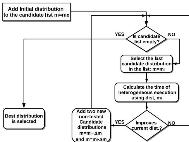
Fig. 6. Flow chart of the Tabu search algorithm for finding the best distribution.
