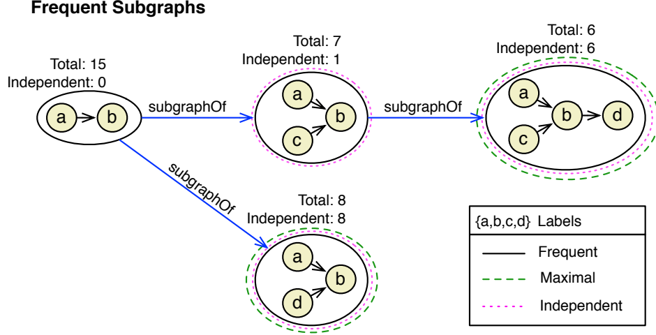
Figure 4: Maximal and Independent Frequent Subgraphs
