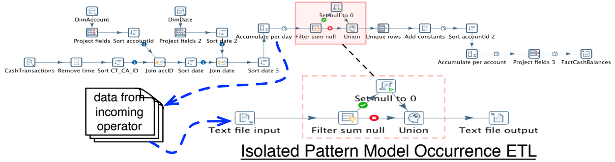
Figure 12: Creating an ETL by isolating a pattern model occurrence
