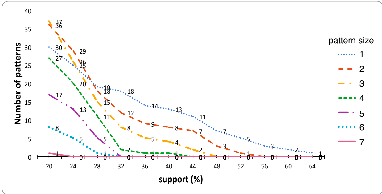
Figure 6: Number of (non-maximal) frequent patterns identified for different support values and for different pattern sizes
