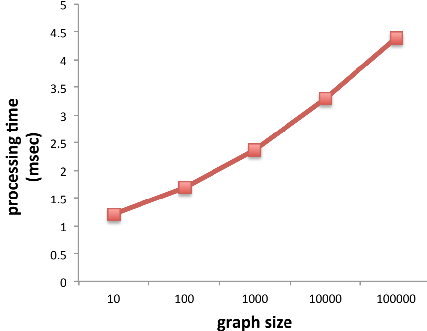
Figure 11: Performance of the graph matching algorithm for ETLs of different sizes (Y-axis in log scale)
