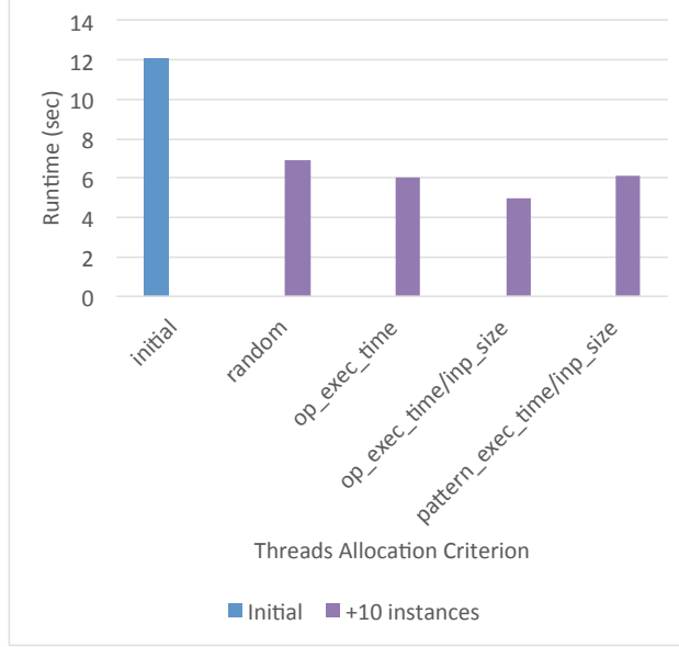
Figure 16: Adding extra instances to Prospect
