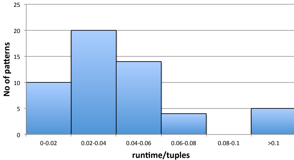
Figure 13: Histogram of number of patterns w.r.t. average values of runtime divided by input size
