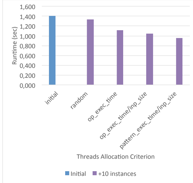
Figure 15: Adding extra instances to DimBroker
