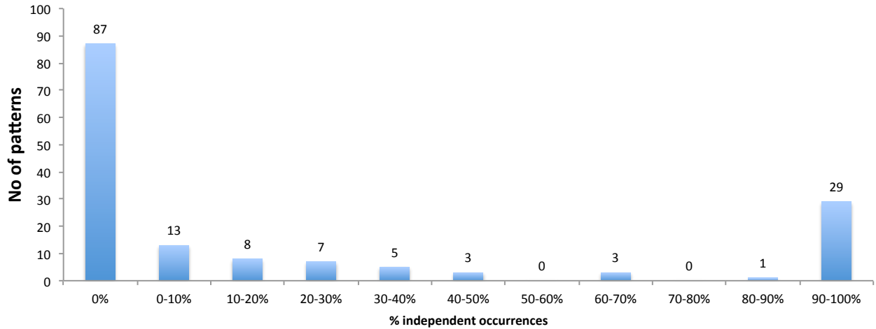
Figure 8: Number of patterns w.r.t. their number of occurrences
