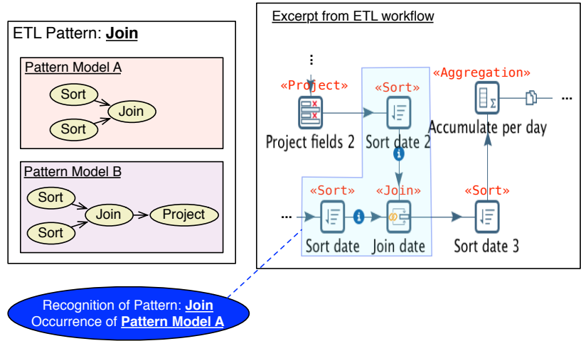
Figure 3: Pattern Model and Pattern Occurrence on an ETL workflow
