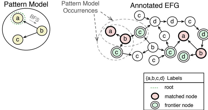
Figure 5: Execution of Find Pattern Model Occurrences Algorithm
