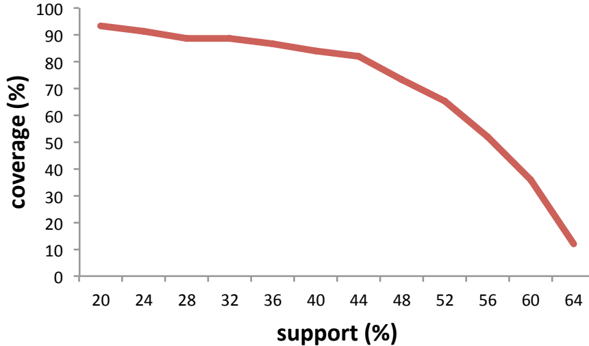
Figure 7: Coverage of ETL workflows for different support values
