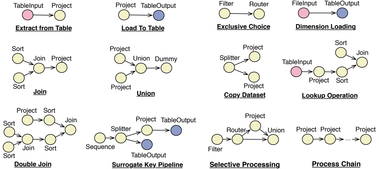
Figure 10: Frequent ETL pattern models
