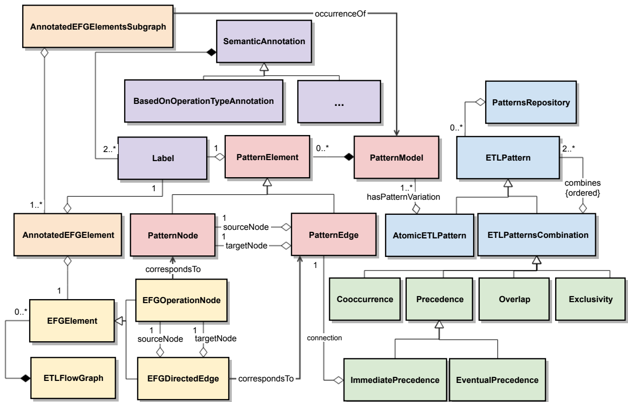
Figure 2: ETL Pattern Conceptual Model
