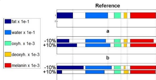
Figure 3. Reference absorbers’ concentrations at the upper subplot (fat concentration 0.5, water concentration 0.7, oxyhaemoglobin concentration 0.002, deoxyhaemoglobin concentration 0.001 and melanin concentration 0.008) and, at the two lower ones, the concentrations obtained by relative fitting a beforehand known forward calculation which represents the spectrally resolved reflectance of a semi-infinite biological tissue. The scattering parameters are constants during the fit and they are fixed with a +10 % or -10 % of error with respect to their real values. The evaluated distance is 4 mm and the thickness of the first layer is 1 mm.
