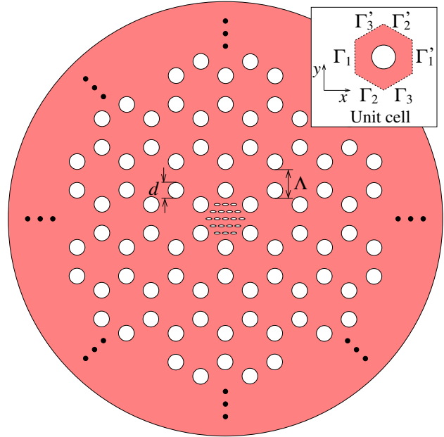
Fig. 1. Honeycomb lattice PBG fiber with an elliptical-hole lattice core (absolutely single-polarization elliptical-hole lattice core PBG fiber). The inset shows the unit cell structure, which was used in calculating the PBG of honeycomb lattices.
