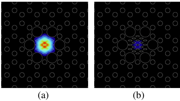
Fig. 8. Field distribution at \Lambda/\lambda = 0.83 in a double single-polarization band PBG fiber after 2 mm of propagation and the light propagation along the fiber of length 2 mm (Supplemental video data: S3.mov and S4.mov). (a) x-polarized beam (S3.mov). (b) y-polarized beam (S4.mov).
