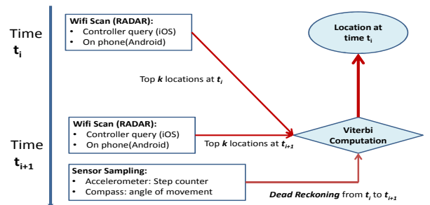
Figure 2. The location estimation algorithm
