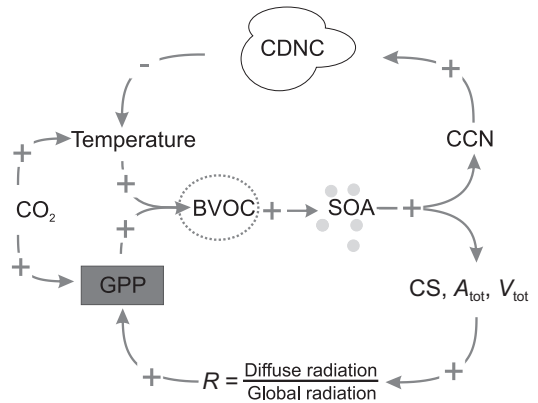
Fig. 1. The two feedback loops associated with the COBACC feedback. Here GPP is the gross-primary production, CS is the condensation sink, A_{\text{tot}} and V_{\text{tot}} are the total aerosol surface area and volume concentrations, respectively, and R is the ratio between diffuse and global radiations. BVOC refers to the biogenic volatile organic compounds, SOA to the secondary organic aerosol, GR_{\text{org}} to the particle growth rate caused by the compounds resulting from BVOC oxidation, CCN to the cloud condensation nuclei, and CDNC to the cloud droplet number concentration.
