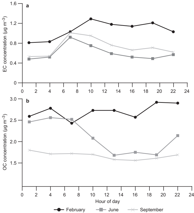
Fig. 4. Average (a) EC and (b) OC and concentrations for eight periods (3-h averages) of day during the measurement campaign (17 June 2006–28 February 2007).
