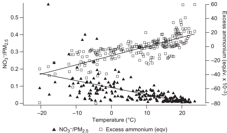
Fig. 7. The nitrate/ PM_{2.5} ratio and amount of excess ammonium as a function of ambient temperature.
