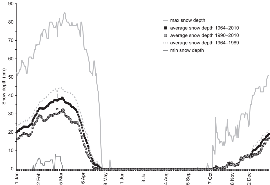
Fig. 4. Temporal evolution of daily snow depth in the course of the year at station 4. In addition to average values for 1964–2010 (black squares), 1964–1989 (dashed curve) and 1990–2010 (grey squares), the highest and lowest values in 1964–2010 are shown.
