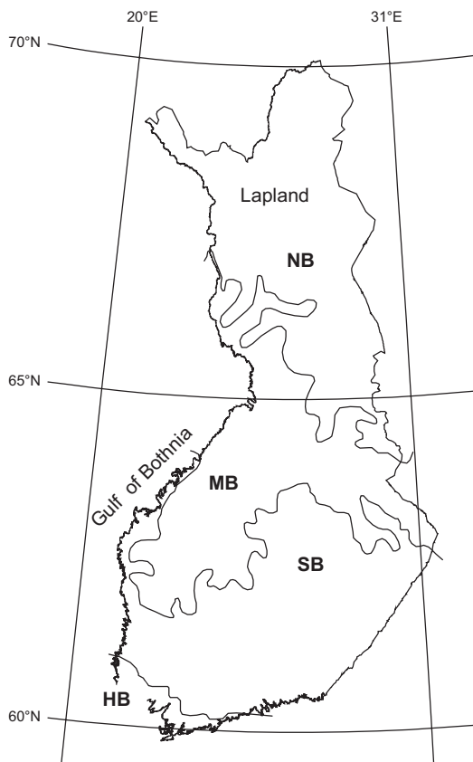
Fig. 1. The study area covered entire Finland. HB, SB, MB and NB are hemiboreal, southern boreal, middle boreal and northern boreal vegetation zones, respectively (Ahti et al. 1968).
