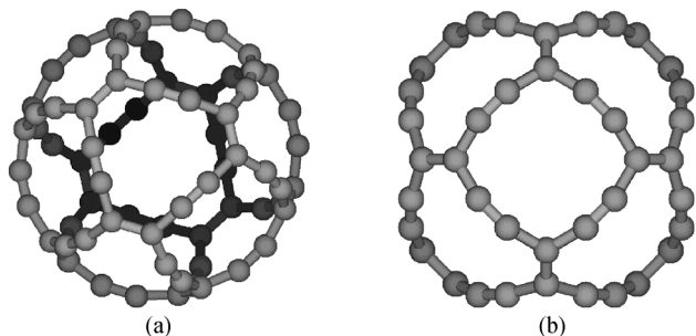
Fig. 1 The molecular structure of gaudiene from two different views. The pictures are made with MOLDEDN. 24
