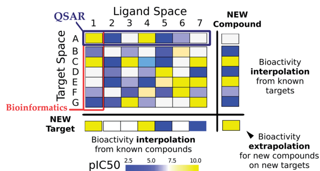
Fig. 1 Ligand–target interaction space. The interaction between ligands (chemical compounds) and targets (biological macromolecules) can be envisioned as a matrix, where rows are indexed by target ids and columns by compound ids. Each matrix cell contains the binding affinity of a given compound on a given target, indicated by the following colors: blue means low affinity and yellow means high affinity. Traditional bioinformatics techniques have dealt with the similarity between targets, normally based upon sequence similarity. On the other hand, ligand based (QSAR) models have studied series of compounds acting on a given target. By contrast to both of them, PCM relates the chemical–target interaction space by describing targets and compounds with numerical descriptors permitting to predict activities of a given compound on a given target.
