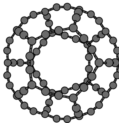
Fig. 3 The molecular structure of \alpha\text{-C}_{80} of I_h symmetry, which is the smallest \alpha -gaudiene investigated.
