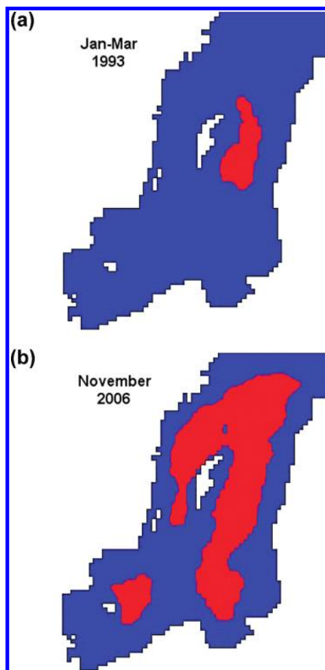
FIGURE 3. Location covered by hypoxic waters containing less than 2 \text{ mL L}^{-1} dissolved oxygen. (A) During its minimum area in 1993 covering 11,050 \text{ km}^2 of bottom and (B) in 2006 covering 67,700 \text{ km}^2 of bottom.
