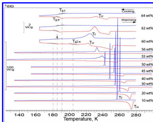
Figure 1. DSC cooling (upper blue lines) and warming thermograms (lower red lines) obtained from 10–64 wt % CA drops at the scanning rate of 3 K/min. Horizontal arrows mark the direction of programmed temperature change. T_f and T_m mark exothermic ice freezing and endothermic ice melting peaks, respectively. T_{g,c} marks a liquid–glass transition upon cooling and T_{g,w} and T_{g2,w} reverse glass–liquid transitions upon warming (see text for details). T_{cr} marks freezing (ice crystallization) upon warming. Solution concentration is indicated. Scale-bars indicate heat flow through samples.
