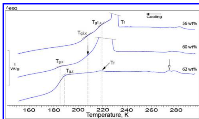
Figure 3. Magnified cooling thermograms of 56, 60, and 62 wt % CA obtained at 3 K/min. The cooling thermogram of 56 wt % CA is from Figure 1. T_{g1,c} , T_{g2,c} and T_{g,c} mark the onset of liquid–glass transitions. A vertical filled arrow marks T_{g2,c} transition in 60 wt % CA thermogram. An open arrow marks a transition from anhydrous CA to CA-monohydrate. 35,36 In the 56 and 60 wt % CA thermograms, the ice freezing peak T_f is truncated to fit the figure.
