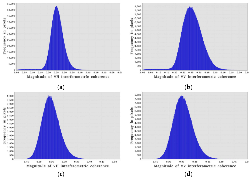
Figure 8. Interferometric coherence histogram for Sentinel-1 image pair on 6 and 18 February 2015 for: (a) VH polarization over the high coherence study area; (b) VV polarization over the high coherence study area; (c) VH polarization over the low coherence area; and (d) VV polarization over the low coherence area.
