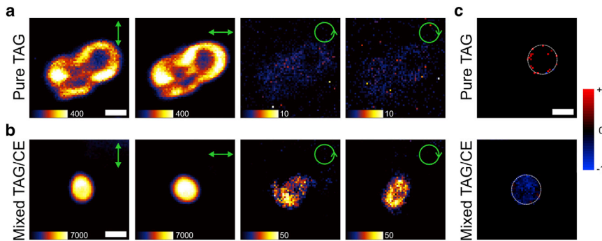
FIGURE 1 Polarized THG microscopy of synthetic LDs consisting of pure TAGs (a) and TAGs and CEs mixed at a 1:1 ratio (b) using orthogonal linear polarizations and opposite-handed circular polarizations at identical experimental settings. The direction of the incident polarization is shown by the arrow. Numbers at the lower left corner indicate the maximum signal level in each image. Scale bar, 2.5 μm. Images for TAG LDs represent a cluster of closely associated LDs. (c) Corresponding THG-CD images of the synthetic LDs. The THG-CD images were derived from the THG images using circular polarizations. The circle highlights the relative position of the imaged LD. For clarity, the spurious CD signals outside the highlighted region are not shown. Scale bar, 2.5 μm. To see this figure in color, go online.
