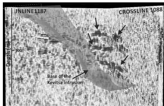
Figure 2. Observed internal reflectivity in the 3D seismic reflection data (Malehmir et al., 2012) within the Kevitsa intrusion. See location of inline 1187 and crossline 1088 from Figure 1. Sections viewed from northwest.
