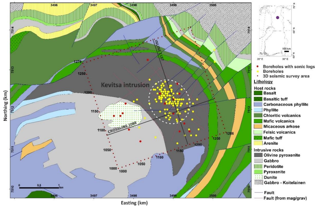
Figure 1. Geological map of the Kevitsa area. Location of the open-pit in dashed white line.
