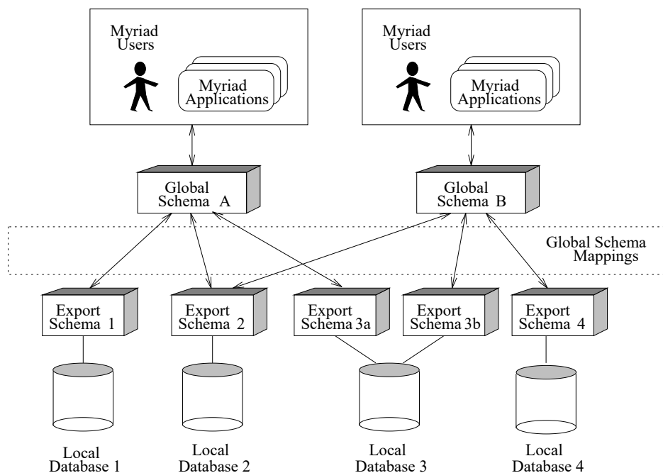
Figure 1. Myriad schema architecture.
