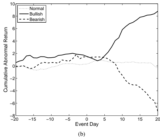
Figure 1: (a) Sample price dynamics of the one-event scenarios. The event is announced in day 160. (b) The cumulative abnormal returns (CAR) for bullish, bearish, and normal (no event) scenarios.
