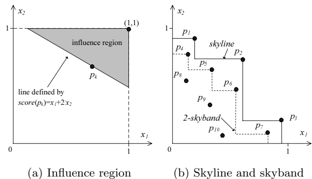
Figure 1: Geometric observations on the top- k problem
