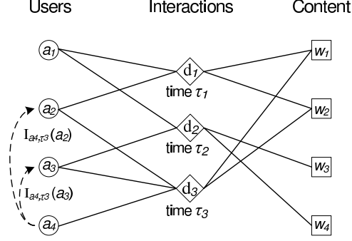
Figure 1: User Interaction Network
