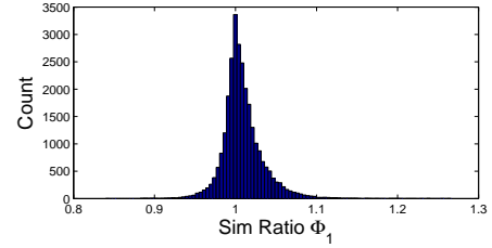
(a) DBLP: Histogram for Sim Ratio \Phi_1(a, t)
