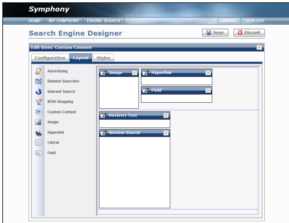
Fig. 1 Design Interface
