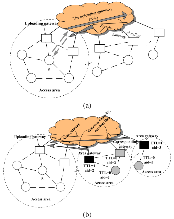
Fig. 4. An example of constructing a two-tier integrated architecture . Square nodes represent gateways. Circle nodes represent mesh routers/mesh clients. Black nodes and gray nodes are the senders and the receivers of AREA_CONSTRUCTION, respectively.
