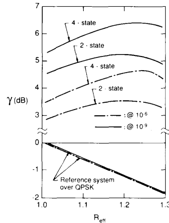
Fig. 3. Coding gain versus R_{\text{eff}} for a concatenated coding system with an R_1 = 8/9 , 6-D TC8PSK inner code and an N = 255 RS outer code with d = 11-61 .
