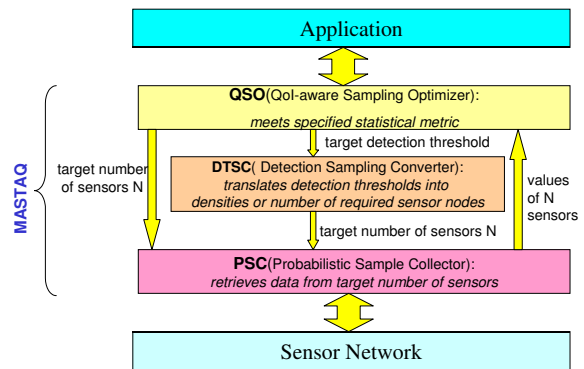
Figure 3. The Architecture of MASTAQ
