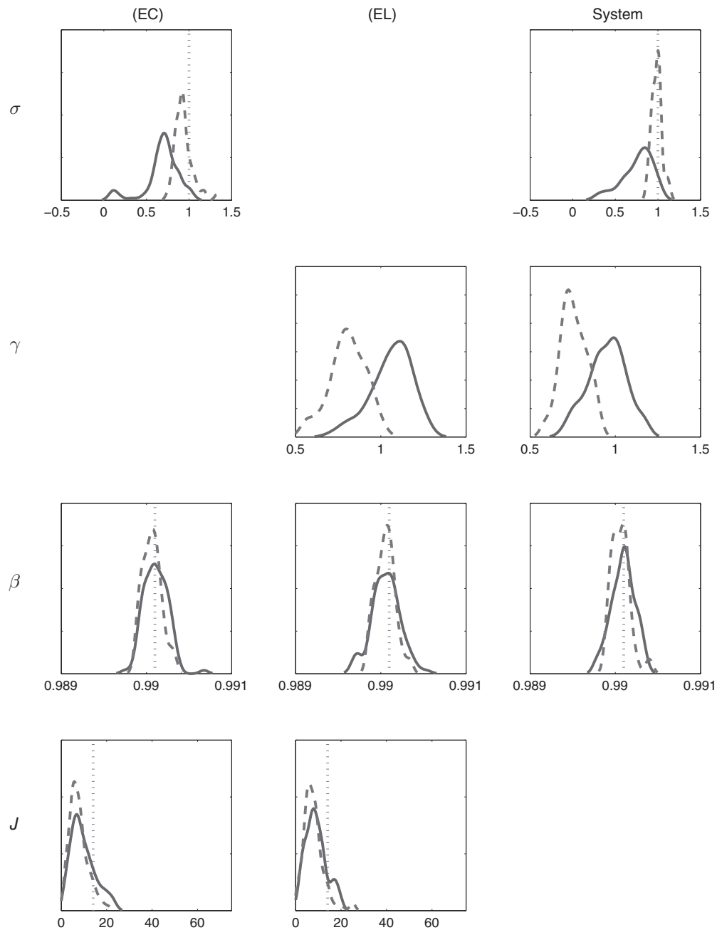
FIGURE 4. KERNEL DENSITY OF PARAMETER ESTIMATES: "INDIVISIBLE-LABOR" MODEL
