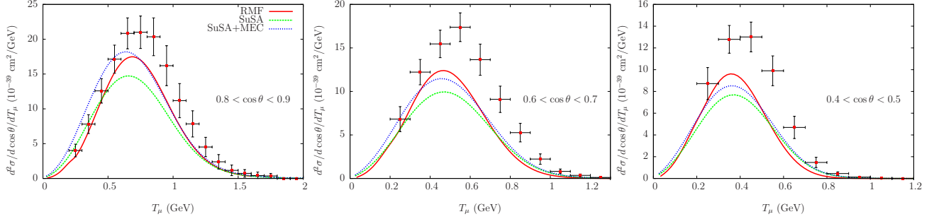
FIGURE 1. Flux-integrated \nu_{\mu} - ^{12}\text{C} CCQE double differential cross section per target nucleon evaluated in the SuSA model with and without inclusion of 2p2h MEC and in the RMF model and displayed versus the muon kinetic energy T_{\mu} for various bins of the muon scattering angle \cos \theta . Here and in the following figures the data are from MiniBooNE [1].
