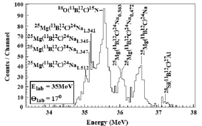
FIG. 3. Energy spectrum for the carbon ( Z = 6 ). The binning is 40 keV/channel.
