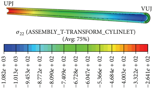
FIGURE 4: Circumferential stresses distribution in solid domain.
