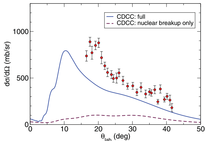
FIG. 13. (Color online) Differential cross section for the angular distribution of transfer/breakup events in ^{11}\text{Be}+^{64}\text{Zn} obtained by selecting ^{10}\text{Be} events in the \Delta E - E spectrum (filled symbols). The solid line is the full CDCC calculation, whereas the dashed line is the CDCC calculation including nuclear breakup only.
