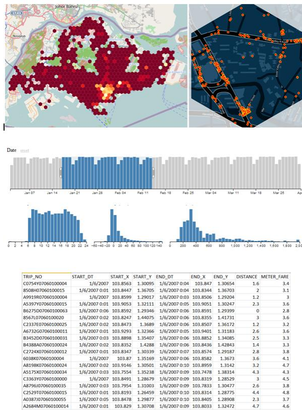
Fig. 5: The interface and components of DIVID.
